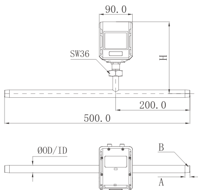
F212x Thread-type dimension schematic
