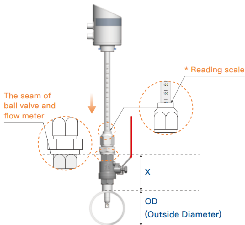
Figure 3-6 Diagram of Insertion Depth Calculation
