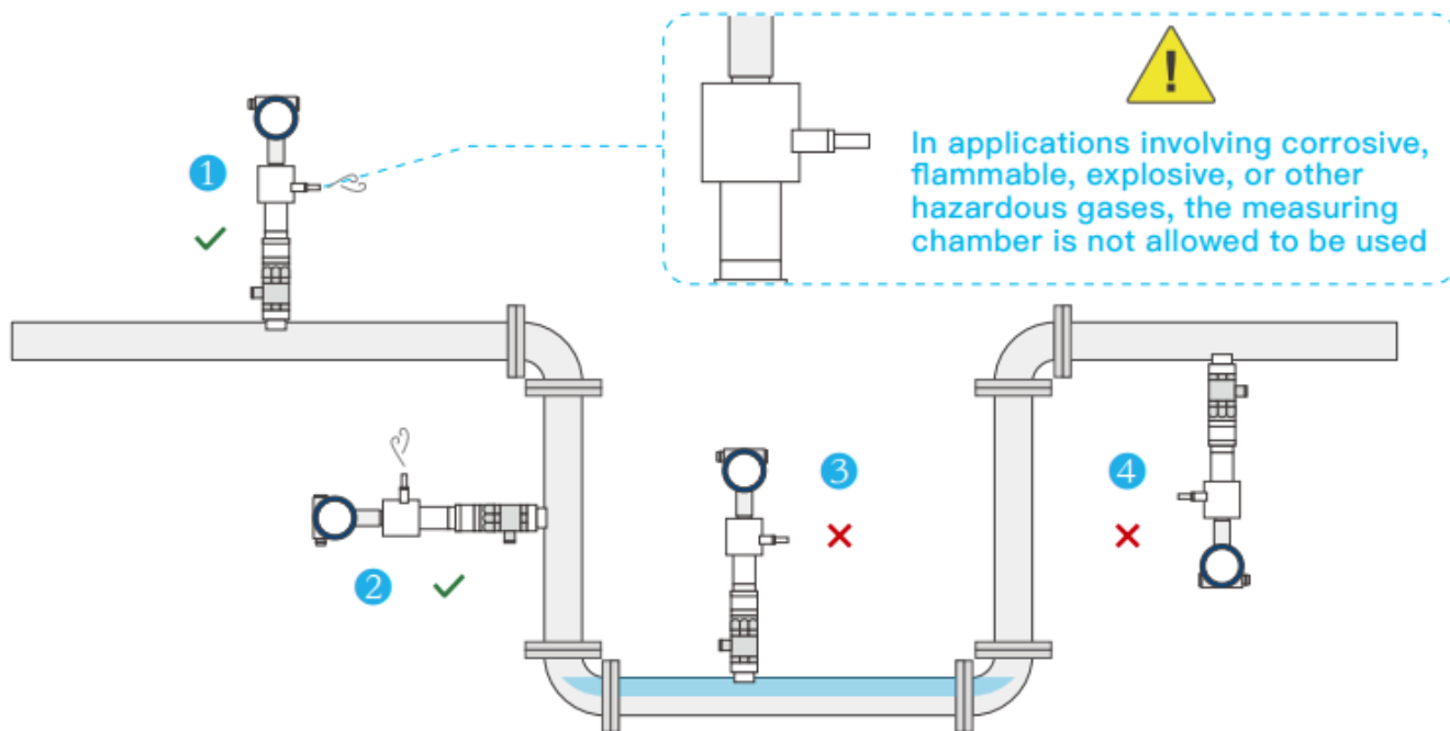
Figure 3-2 Installation with Measuring Chambers
