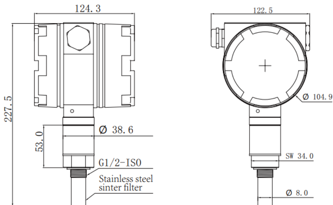
Figure 3-1 F191x-Ex Series Dimension Diagram
