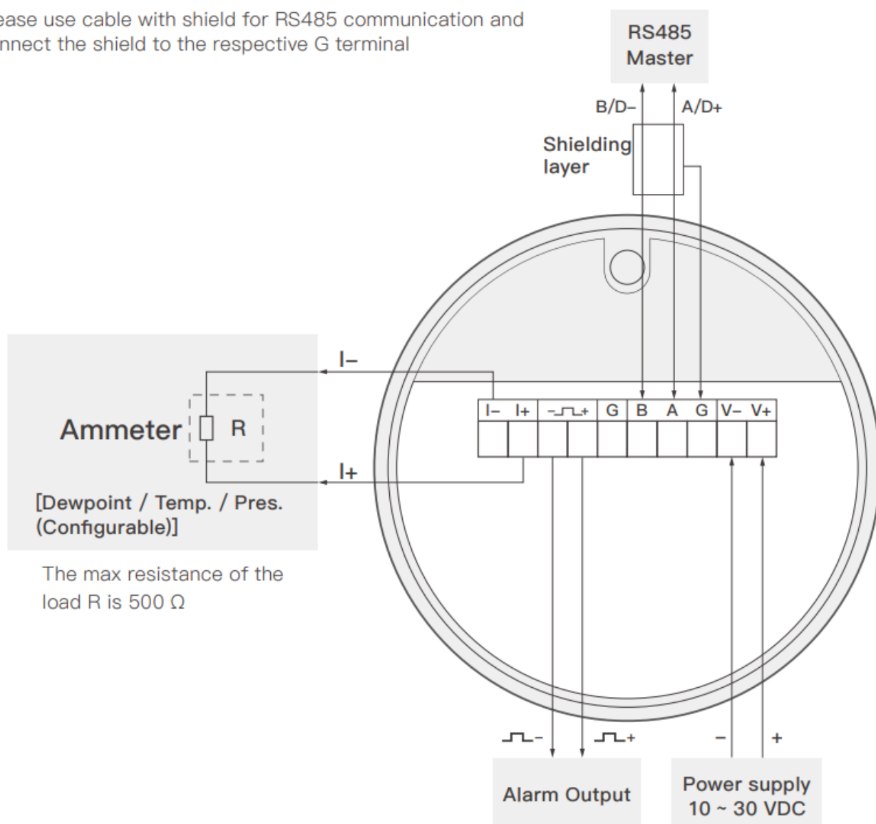
Figure 3-5 Electrical Connection Diagram
