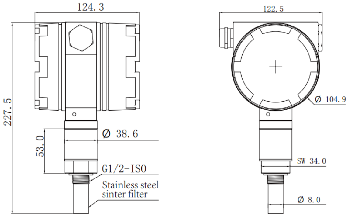
Figure 3-1 F103x Series Dimension Diagram
