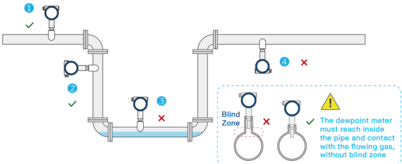
Figure 3-3 Installation Directly on the Pipe
