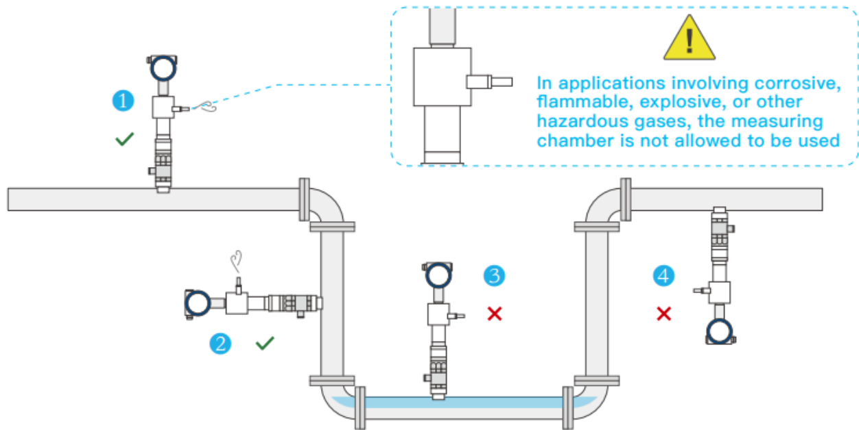
Figure 3-2 Installation with Measuring Chambers
